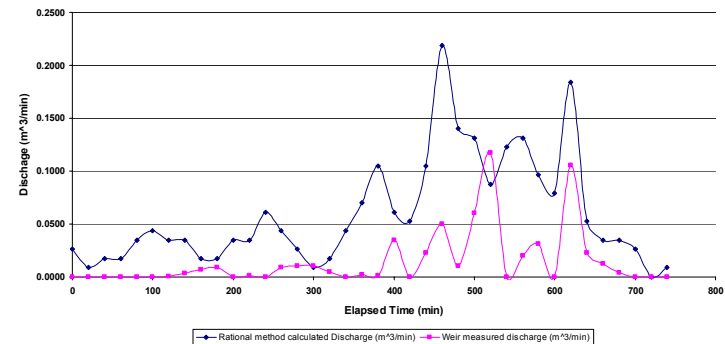
Brookes 9/27/02 Rational method calculated hydrograph (shifted 60 minutes to observed peak discharge) and weir measured discharge
