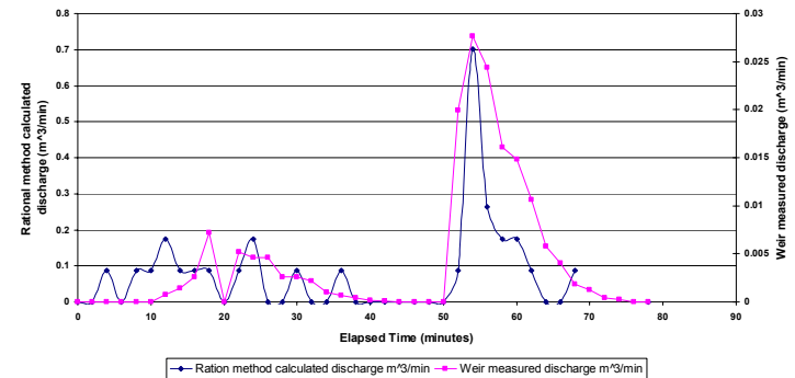
Brookes 9/11/02 Rational method calculated hydrograph (shifted 4 minutes to peak observed discharge) and Weir measured discharge
