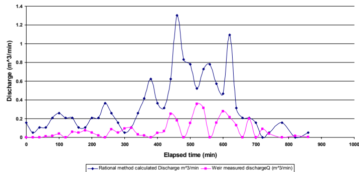
Perkins 9/27/02 Rational method calculated hydrograph (shifted 60 minute to peak observed discharge) and weir measured discharge.
