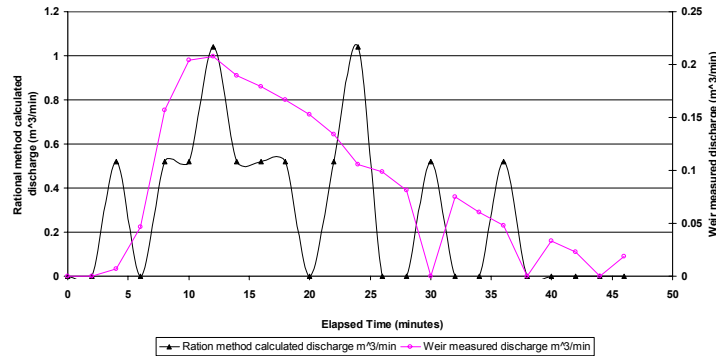
Perkins 9/11/02 Rational method, calculated, hydrograph (shifted 4 minutes to observed peak discharge) and weir, measurement generated, hydrograph
